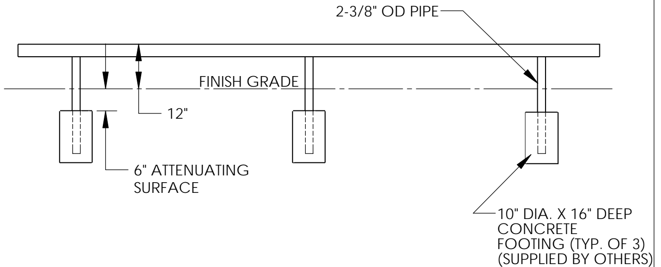
ELEVATION VIEW
