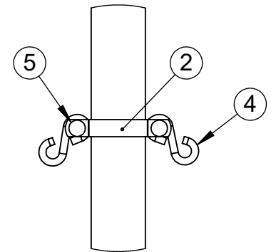
DETAIL B
