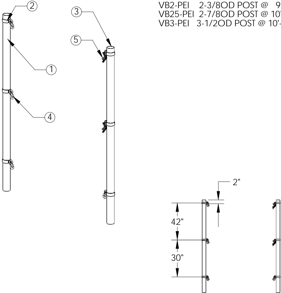
ELEVATION VIEW
