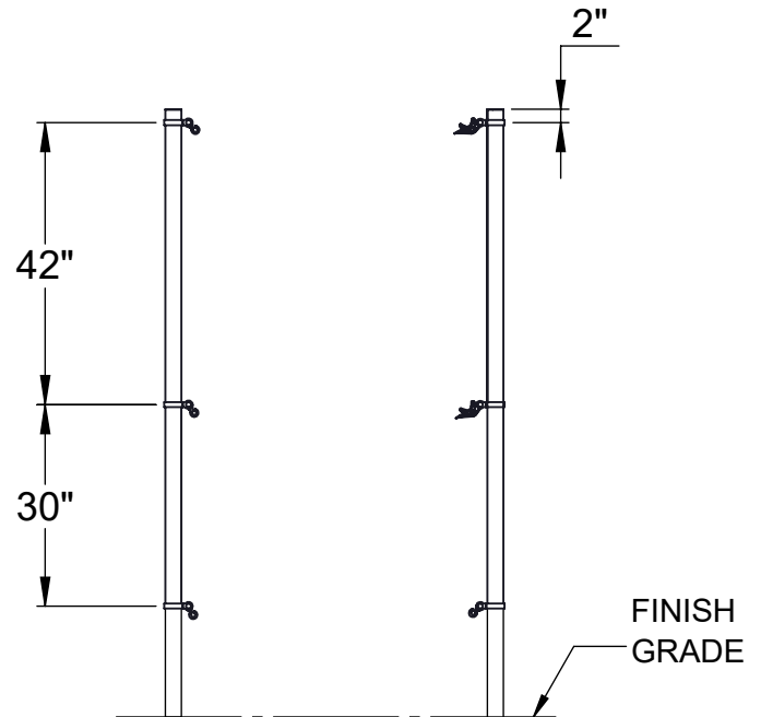
ELEVATION VIEW
