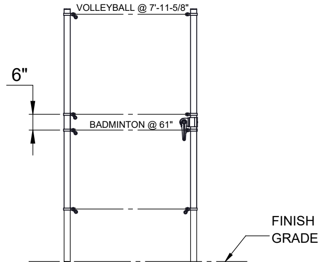
NET HARDWARE DETAIL/ELEVATION
