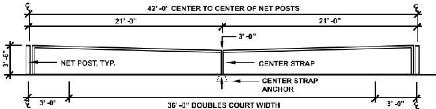
Typical Tennis Net Elevations
