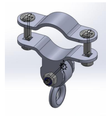
2 3/8" SWING HANGER
