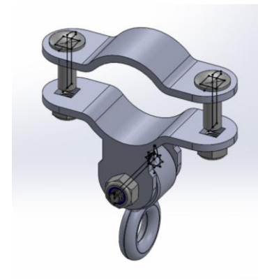
2 3/8" SWING HANGER
