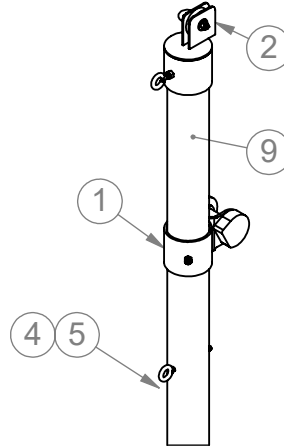
(1) 2202-11-TP -1 EYEBOLT/NYLOCK- -TOP PULLEY- -NET TIGHTENER-
