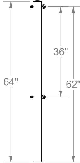
(1) 2202-11 2 EYEBOLT/NYLOCK
