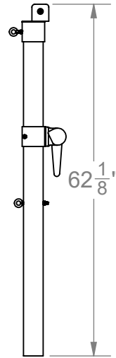
(1) 2202-11-TP -1 EYEBOLT/NYLOCK- -TOP PULLEY- -NET TIGHTENER-
