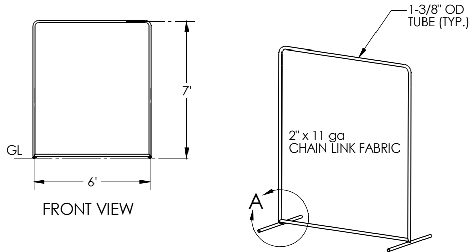
FPS-N BASEMANS PROTECTION SCREEN
