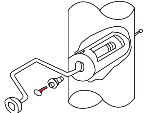
Winch Detail
