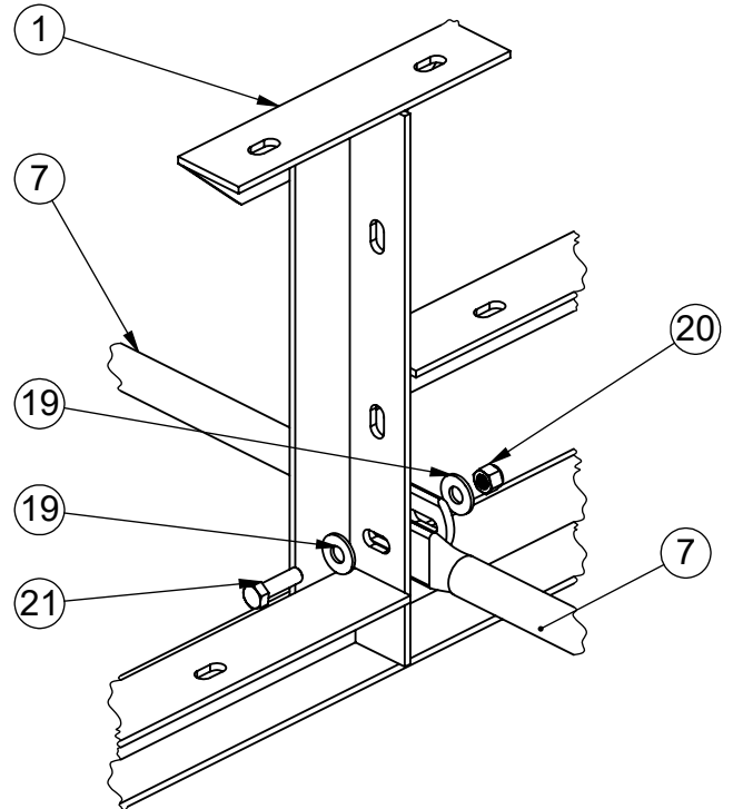
DETAIL D ENLARGED FROM SHEET #7 SCALE 1 : 5
