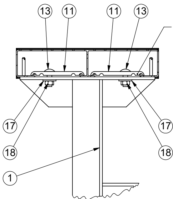
DETAIL I ENLARGED SCALE 1 : 4
