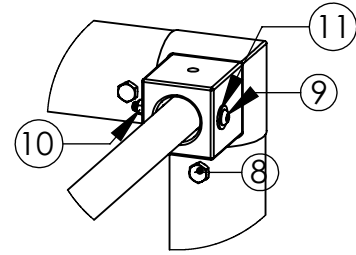
DETAIL H
