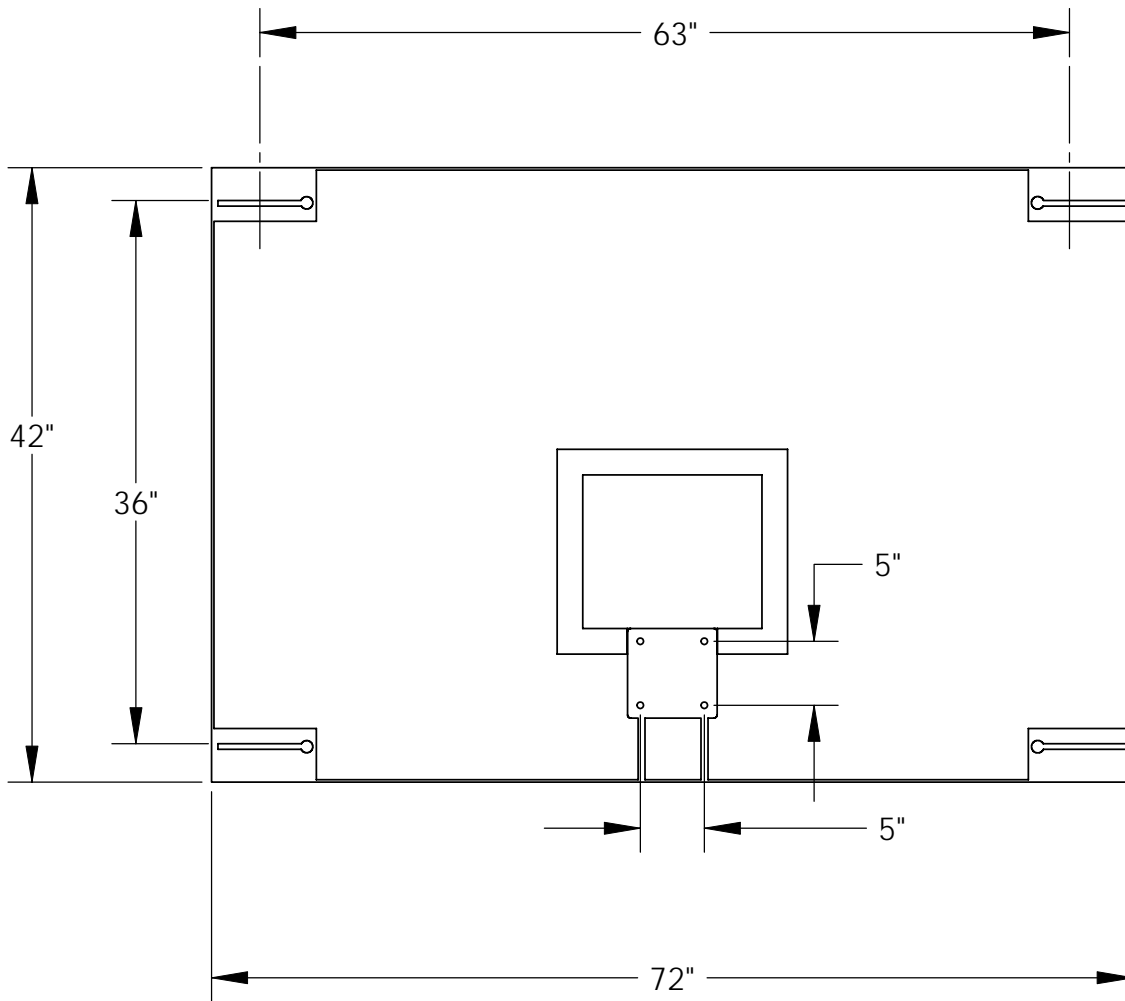
BACK VIEW
