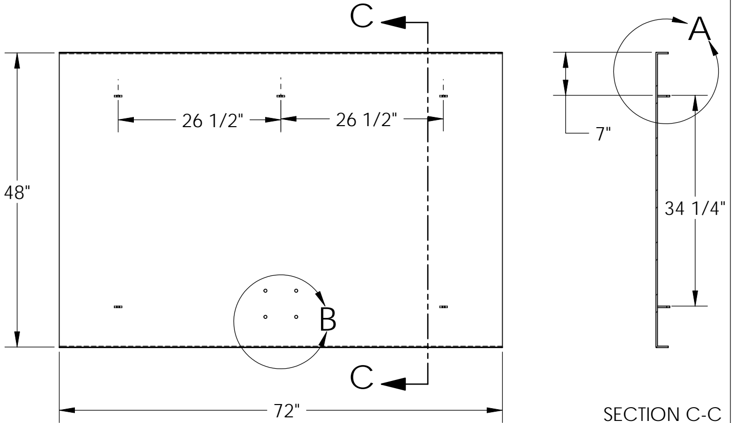
BACK VIEW
