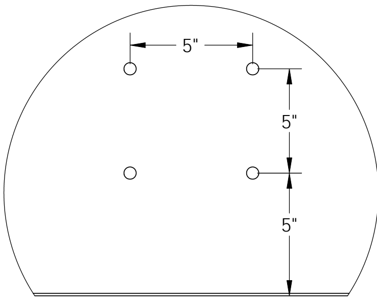
DETAIL B
