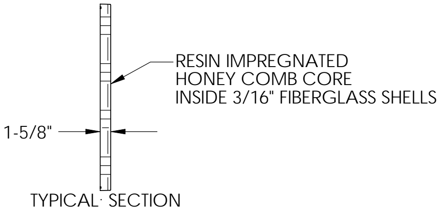
-05 BASKETBALL BACKBOARD
