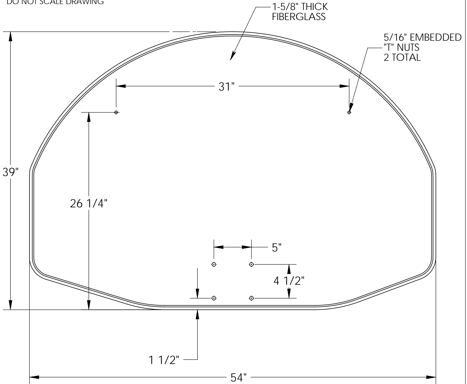
-05 BASKETBALL BACKBOARD
