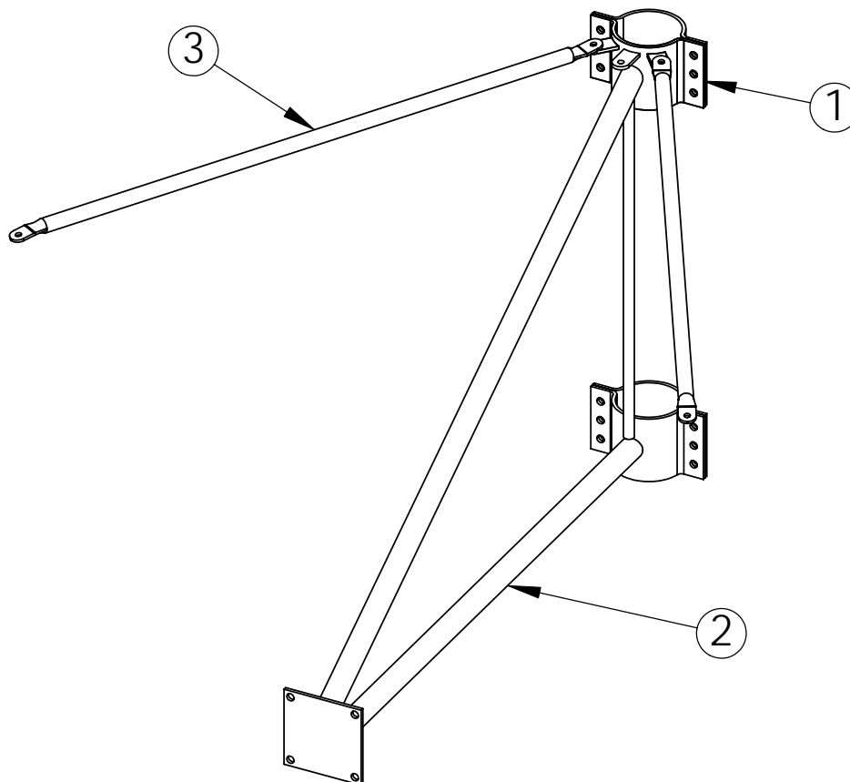
ZE-44 EXTENSION FRAME
