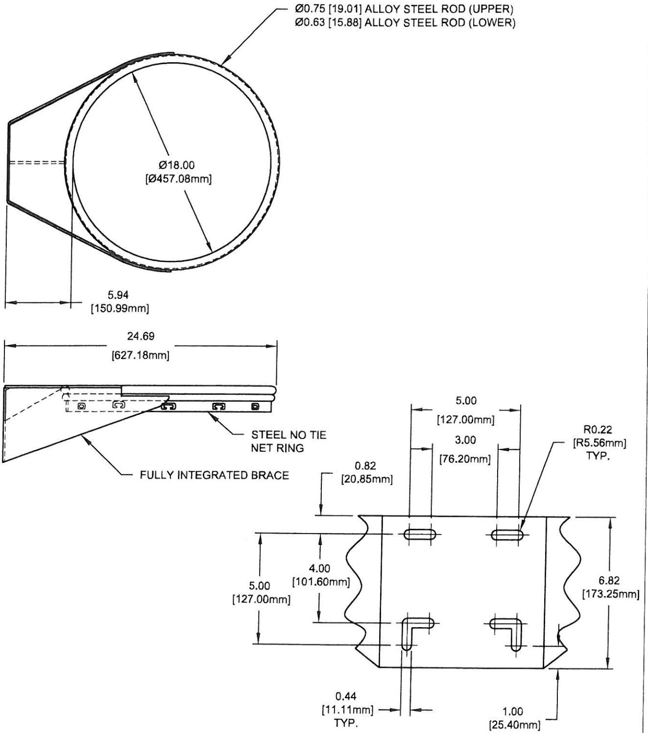
MOUNTING PLATE VIEW
